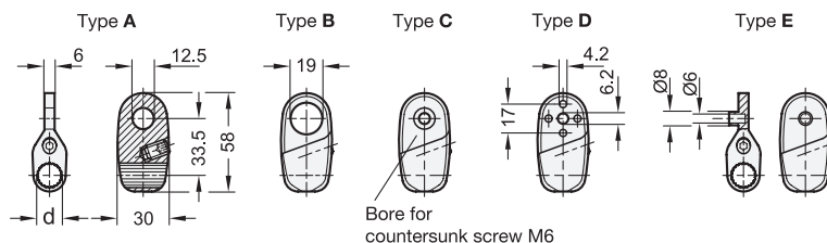
GN 177.1 (Work gripper blocks)
