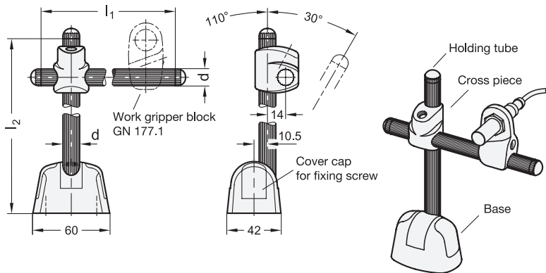
GN 177.1 (Work gripper blocks)
