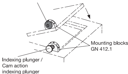
Positioning bushing with ramping cone GN 412.3 / GN 412.5
