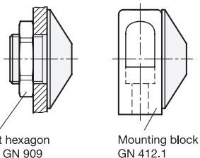
Assembly examples
